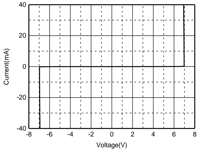
I-V Curve
